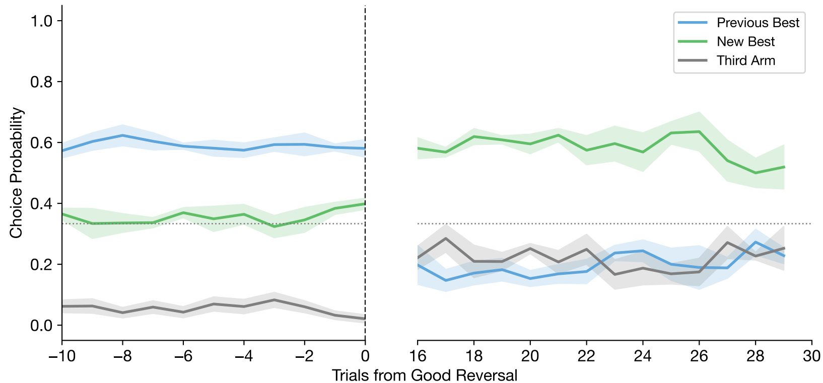
Good Reversal-Aligned Choices (mean \pm se across subjects | n=5 subjects, n=85 reversals) (Skipping first 15 trials post-reversal)
